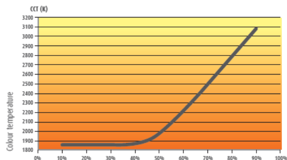
Dimmer curve, Luminosity vs Colour Temperature
