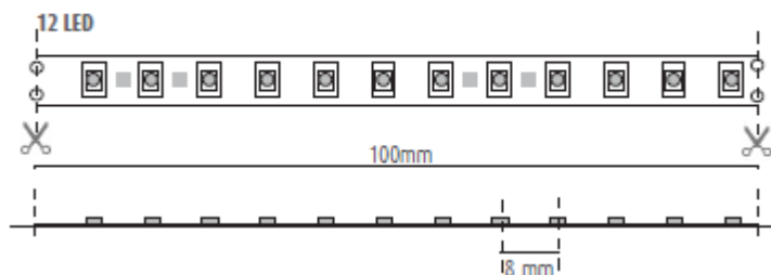
LED SPACING AND PITCH CUT
